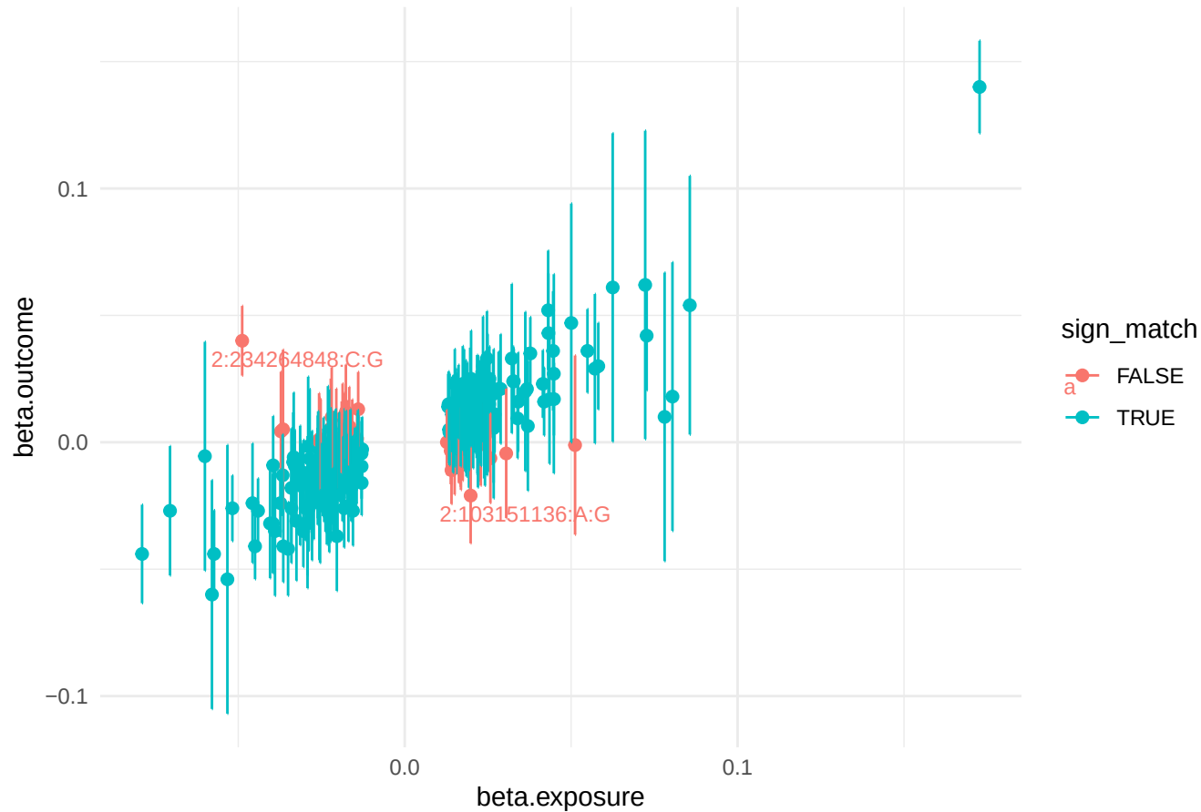
Exposure vs Outcome betas; discordant SNPs labeled
